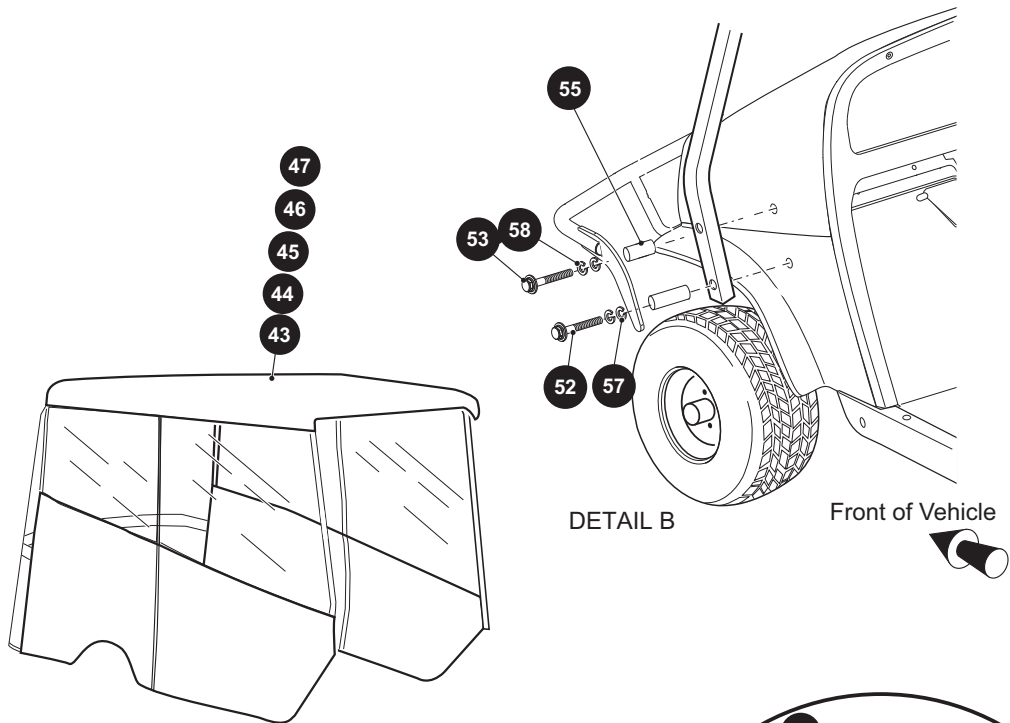
WEATHER ENCLOSURE
